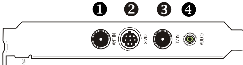
Figure 2–2 ATI TV Wonder™ 650 PCIe Backplate
